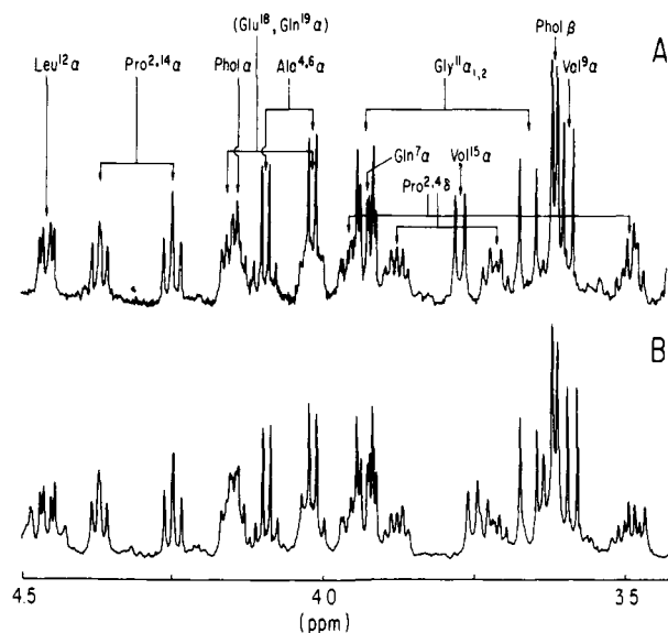
Figure 5. The 600-MHz ^1\text{H} NMR spectra of the C_\alpha -H region of synthetic (A) and natural (B) alamethicin I. The spectra were taken in methanol- d_4 at a concentration of 1–2 mg/mL and at a temperature of 23^\circ\text{C} . Line assignments (in ppm relative to TMS) are based on splitting patterns, comparison with spectra of synthetic segments, and double resonance difference spectra (cf. ref 38). The upfield shift (0.02 ppm) and twofold broadening of the Val 15 C_\alpha -H signal at 3.75 ppm in B is accounted for by differences in concentration and water contents of the two samples. Thus, dilution and addition of \text{D}_2\text{O} ( \sim 2\% ) to B caused the line to sharpen and shift downfield.
