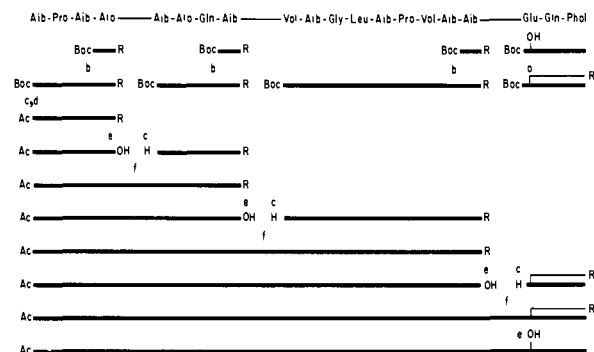
Figure 2. Scheme of the synthesis of alamethicin I by solid-phase segment condensation (R = resin). Procedures and reagents (see Experimental Section for details): (a) \text{CsHCO}_3/\text{DMF} ; (b) stepwise chain elongation; (c) (1) TFA, (2) DIEA; (d) \text{Ac}_2\text{O} ; (e) HF followed by purification; (f) DCC-HOBt.
