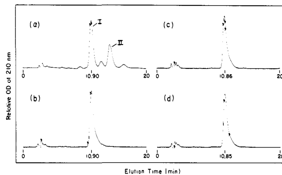
Figure 3. Reversed phase high performance liquid chromatography of natural and synthetic alamethicins. Column, 0.46 × 25 cm Partisil 5 ODS (Whatman); flow rate, 1.2 mL/min; eluent, methanol (85%)/2 × 10 -2 M aqueous triethylammonium acetate pH ~5 (15%); samples ca. 10 μg in ethanol-water (1:1). (a) Natural alamethicin (Upjohn) containing the two major components I and II. (b) Isolated natural alamethicin I. (c) Synthetic alamethicin I. (d) 1:1 mixture of natural and synthetic alamethicins I.
